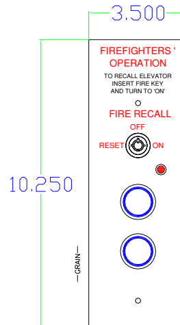
Intermediate Hall Station with 2007 Fire Service (Note height increase to allow engravings per code. Site conditions should be verified)
