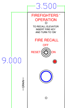
Terminal Hall Station with 2007 Fire Service
