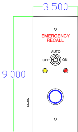
Terminal Hall Station with 1998 Fire Service
